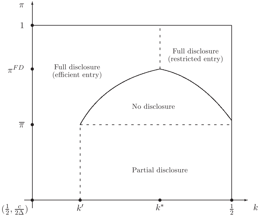
OPTIMAL DISCLOSURE POLICY AS A FUNCTION OF k AND \pi
